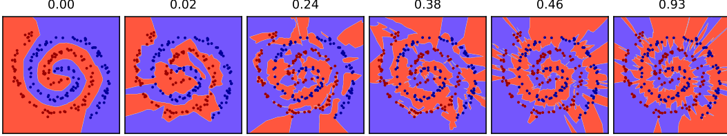
Figure 6: Swissroll decision boundary for various levels of generalization gap (indicated above plots).
